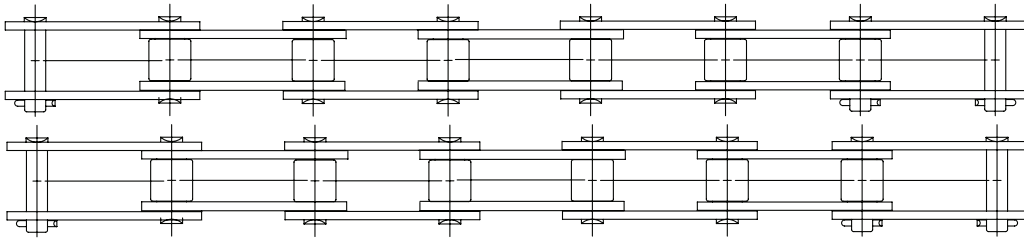
Double Pitch Top View
